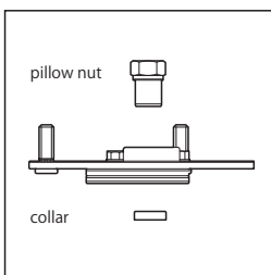
①Pillow Upper Mount for Strut:Adjustable for SA:Non-Adjustable
