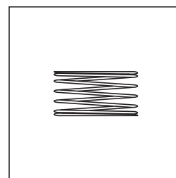
④Helper Spring (1.9kgf/mm) ⑤Helper Spring (0.5kgf/mm)
